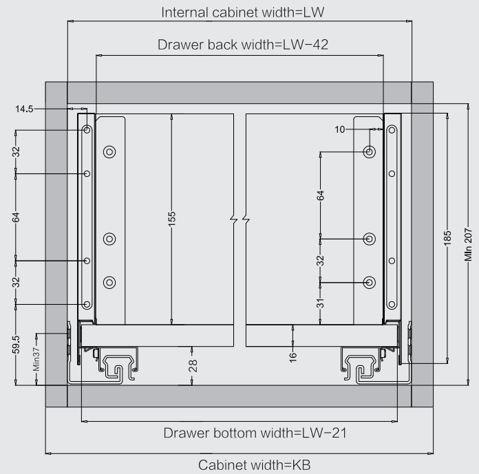
LW Internal cabinet width
