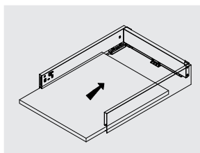
Bottom assembly
